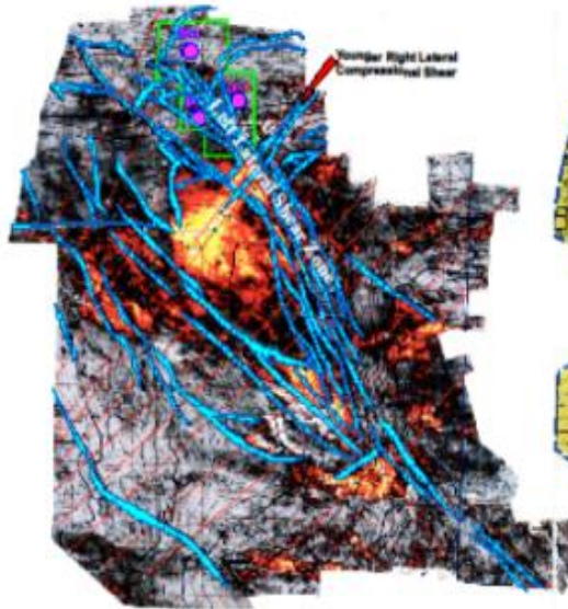
(A.) Beneath the Jurassic Unconformity (The hydrocarbon kitchen)
